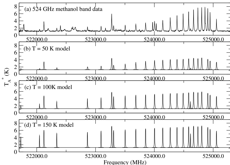
Fig. 6. Modeled spectra compared with the those observed in the 524 GHz methanol band (panel a), for models with constant temperature of 50 (panel b), 100 (panel c), and 150 K (panel d), assuming the compact ridge is a spherical clump 5'' in radius ( r ), constant molecular hydrogen number density 10^7 \text{ cm}^{-3} , and methanol abundance 10^{-6} .
