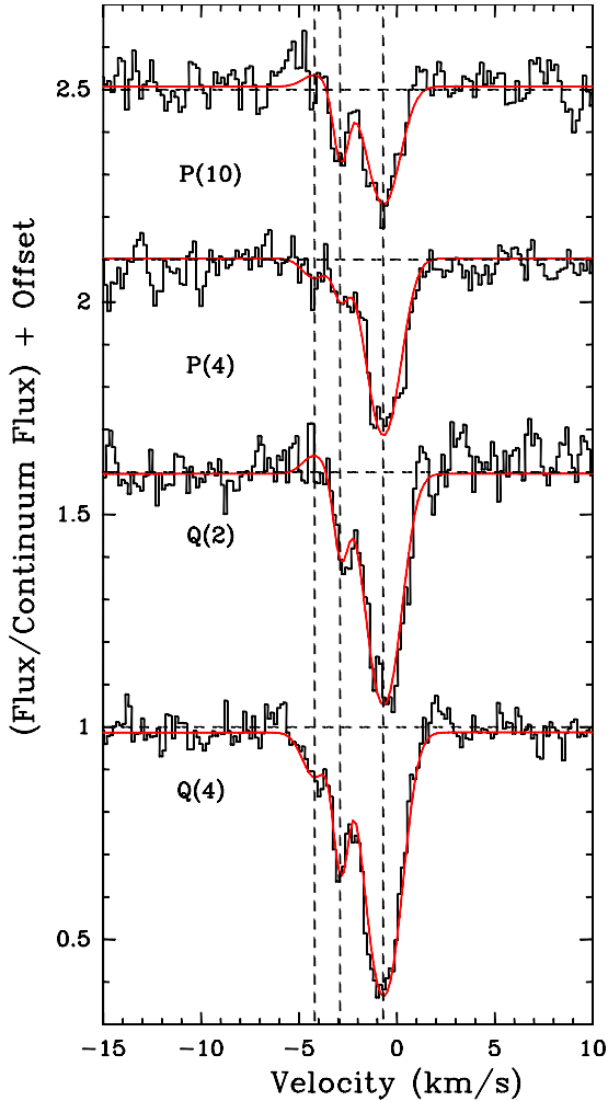
Fig. 1. HIFI observations of the C_3 lines in DR21(OH). The spectra are corrected for the DSB continuum and normalized to the SSB continuum level. The Q(2) , P(4) , and P(10) spectra are shifted consecutively by +0.5, so that the plots do not overlap. The red line shows the simultaneous fit with three Gaussian velocity components (at -0.7 , -2.9 , and -4.2 \text{km s}^{-1} ). Note that the third component is only detected above the noise in Q(4) and P(4) . The “negative” absorption bumps at this velocity fitted in Q(2) and P(10) are within the noise.
