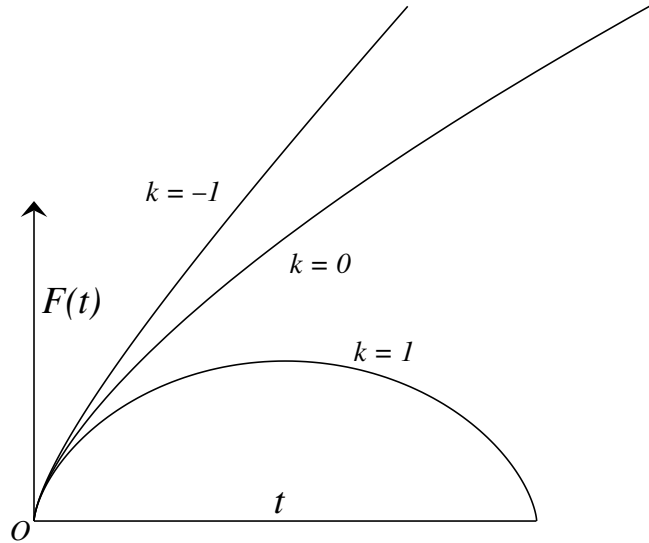
Fig. 6. The Robertson-Walker universe with \Lambda = 0 , for k = 1 , k = 0 , and k = -1 .
