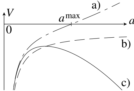
Fig. 5. The potential (14.20) for the cases a) k = 0, \Lambda < 0 , b) k = -1, \Lambda = 0 and c) k = 0, \Lambda > 0 . In the case (a), there is a turning point at a = a^{\max} .
