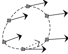
Fig. 3. Parallel displacement along a closed curve in a curved space.
