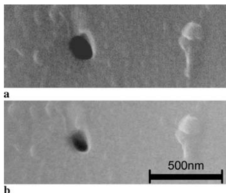
FIGURE 4 (a) Hole in the AFM tip, before ion-implantation procedure; (b) after ion-implantation procedure of Ar and N with a dose of 4 \times 10^{16} ions/cm 2
