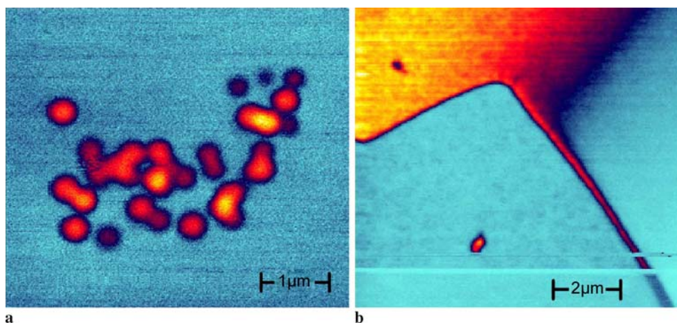
FIGURE 5 (a) A group of NV centers produced by MeV implantation using a nanoprobe implantation system. (b) A NV center produced by the nano-addressing system with an ion gun having an ion kinetic energy of 2 keV
