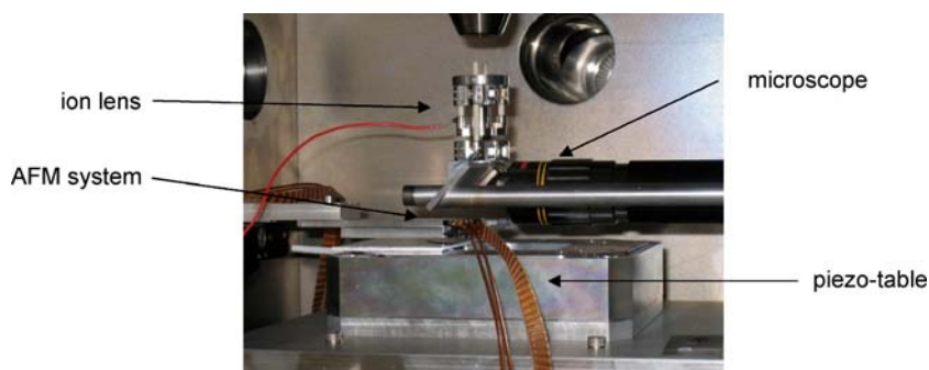
FIGURE 2 A view inside the nano-addressing chamber
