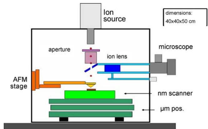
FIGURE 1 From top to bottom: the ion gun providing different kinds of ions, a micro ion lens with apertures, an optical microscope with a pierced mirror and a table with sub-nm resolution. The pierced AFM tip can be moved precisely in all directions using micromotors. The target is based on a PI piezo table with 0.1-nm resolution and a stepping motor driven table for \mu\text{m} alignment
