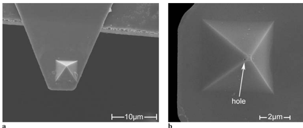
FIGURE 3 (a) Glued hollow AFM tip with piezoresistive cantilevers. (b) Hole drilled into AFM tip using a focused ion beam (FIB)
