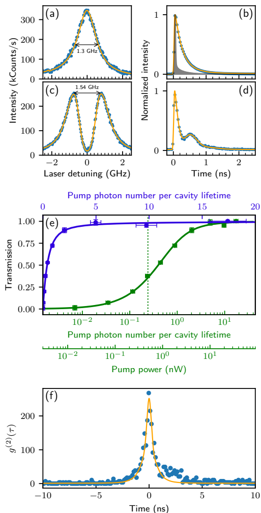
FIG. 2. Transmission spectrum of the bare cavity (a) and the coupled molecule-cavity system (c). Ring-down temporal signal of the bare cavity (b) and the coupled molecule-cavity system (d). The fits to the experimental data (solid orange curves) take the detector response function (shown by the grey area in (b)) into account. (e) Transmission through the cavity on resonance with the molecule and the laser as a function of the excitation power. Green and blue present the same data for different horizontal axis scalings. The vertical dotted line marks S = 1 . (f) Intensity autocorrelation of the light transmitted through the cavity on resonance with the molecule and the laser. The maximum value of 250 is limited by residual background light, which was accounted for by the theoretical fit (orange curve).
