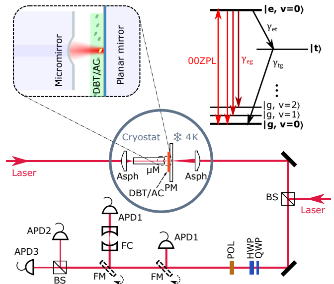
FIG. 1. Schematics of the experimental setup. Details can be found in Refs. [16, 17]. An external Fabry-Perot cavity (FC) serves as a narrow-band filter for the molecular emission. BS: beamsplitter, Asph: aspheric lens, \mu\text{M} : micromirror, PM: planar mirror, DBT/AC: dibenzoterrylene-doped anthracene crystal, QWP: quarter-wave plate, HWP: half-wave plate, POL: polarization filter, FM: flip mirror, APD: avalanche photodiode. Left inset: A close-up of the microcavity. Right inset: Jablonski diagram for DBT. The 00ZPL takes place at a wavelength of \lambda \sim 785 nm. The triplet state is denoted by |t\rangle .
