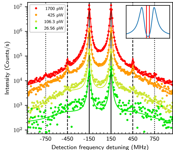
FIG. 3. Transmission spectrum of the coupled system under excitation at two frequencies separated by 300 MHz at different powers (see legend) The spectra reveal the generation of higher harmonics. The theory curves reproduce the features. The vertical lines point to the regular frequency spacing of the observed signals.
