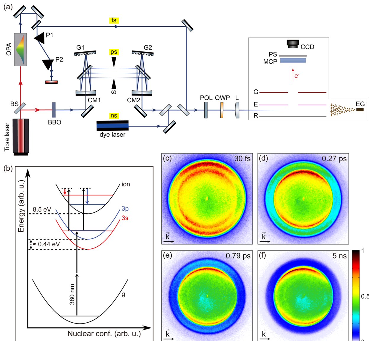
Fig. 1 (a) Schematic diagram of the experimental setup. To generate femtosecond, picosecond, and nanosecond laser pulses centered at 380 nm, we used an optical parametric amplifier, the second harmonic output of a Ti:sapphire laser followed by a 4f pulse shaper, and a tunable dye laser. After controlling the polarization, the pulses were focused in the VMI spectrometer to interact with fenchone molecules supplied as effusive gas (EG). Photoelectrons from the interaction region were then amplified by the microchannel plates (MCP) and imaged on a phosphor screen. A CCD camera was used to accumulate the image on the phosphor screen. (b) 2 + 1 REMPI scheme of fenchone with 380 nm ( \approx 3.26 eV) radiation. There are two intermediate resonances in the 2 + 1 REMPI scheme, namely 3s and 3p. The energy difference between the lowest edge of the two intermediate resonances is about 0.44 eV. 28,31 As illustrated in the figure, the final ionization step does not change the vibrational levels according to the \Delta v = 0 propensity rule for parallel potential surfaces. (c–f) Raw photoelectron angular distributions (PADs) measured with S-(+)-fenchone by using LCP pulses with (c) 30 fs, (d) 0.27 ps, (e) 0.79 ps, and (f) 5 ns duration. The light propagation directions are left to right for all PADs and indicated with arrows on the PADs. Each PAD comprises two concentric circles. The inner circle corresponds to photoelectrons via the 3s intermediate, and the outer circle corresponds to the 3p intermediate. The influence of internal conversion is shown from PADs (c–f) as fading of the outer circle.
