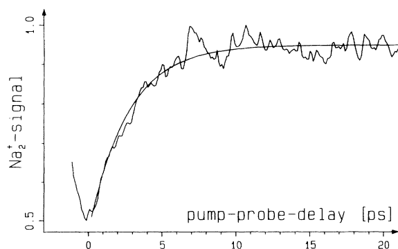
FIG. 3. Transient cluster photofragmentation spectrum showing the buildup of “fast” neutral dimer fragments \text{Na}_2 photoionized by the probe laser. The corresponding time constant is 2.5 ps. The strong photoinduced fragmentation doubles the total \text{Na}_2^+ signal within 10 ps.
