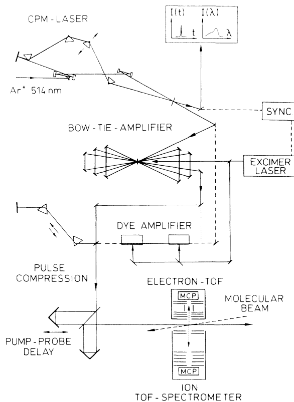
FIG. 1. Femtosecond pump-probe laser system and molecular beam arrangement. Femtosecond pulses ( t = 60 fs) are generated by a colliding-pulse mode-locked (CPM) ring dye laser, amplified in dye amplifiers, pulse compressed, and split into identical pump and probe pulses. Pump and probe laser beams are collinear and perpendicular to the molecular beam and the TOF spectrometers.
