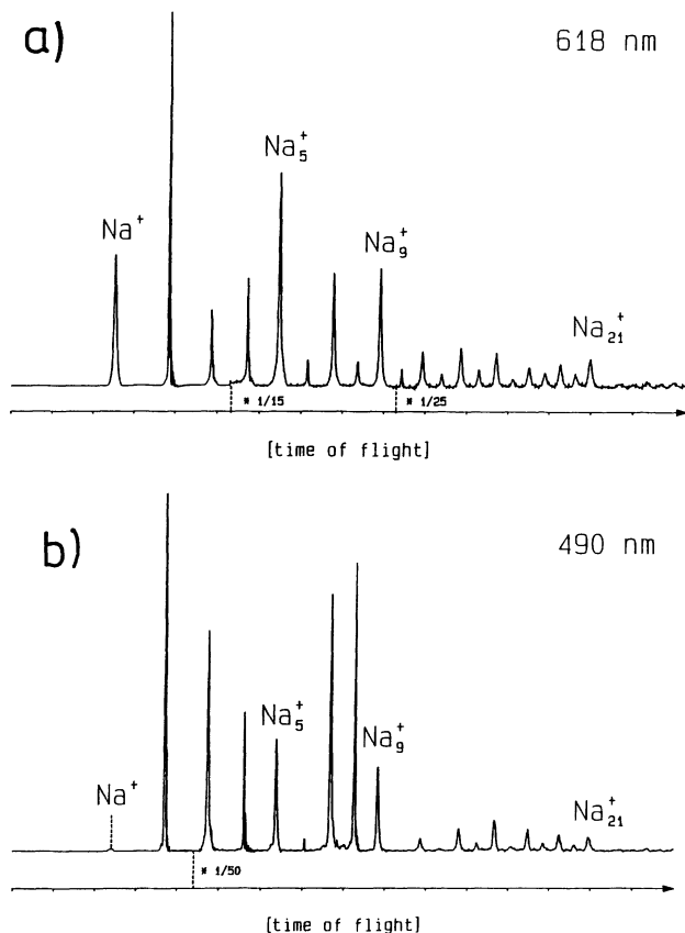
FIG. 2. Sodium cluster ion \text{Na}_n^+ mass spectra resulting from the interaction of a femtosecond laser pulse of 60-fs duration and of a 1- \mu\text{J} pulse energy with a sodium cluster beam. The spectra (a) \lambda_{\text{max}}=618 nm and (b) \lambda_{\text{max}}=490 nm are obtained under the same conditions. The individual cluster ion intensities for n \leq 9 strongly depend upon the wavelengths used, whereas they do not for n=10 –21.
