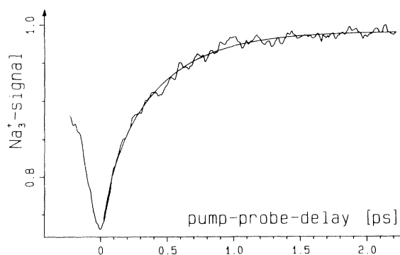
FIG. 4. Pump-probe delay spectrum of the ejected neutral trimer fragments \text{Na}_3 . The probe signal \text{Na}_3^+ buildup time constant of 0.4 ps indicates a direct photoinduced fragmentation of sodium cluster ions rather than a statistical unimolecular decay.
