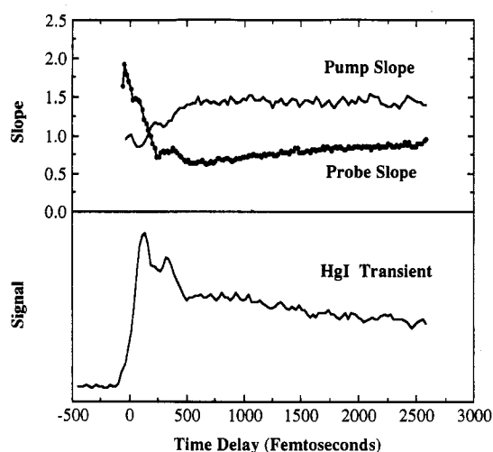
Figure 2. (bottom) The femtosecond \text{HgI} transient. Two sharp peaks separated by 220 fs are followed by a broad peak at about 1 ps and by a nonzero asymptote. (top) The pump slope increases from 0.95 \pm 0.1 to a constant value of 1.45 \pm 0.1 at 500 fs. In the rising part of the pump slope there is a noticeable dip at the position of the second peak in the transient. The probe dependence mirrors the pump dependence: it drops from a slope of more than 1 to a minimum at 500 fs of 0.6 \pm 0.1 (some saturation) but then rises again toward 1.
