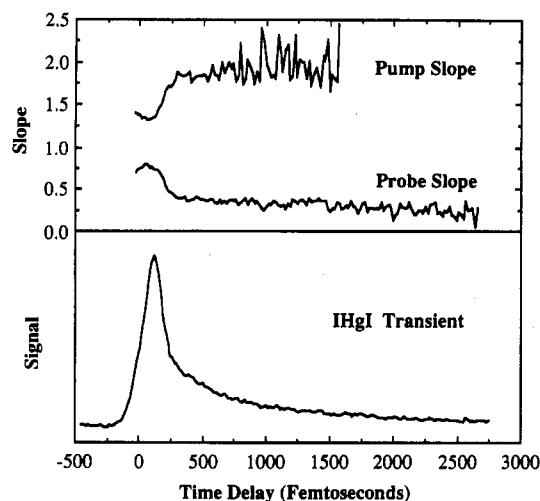
Figure 1. (bottom) The femtosecond \text{HgI}_2 transient which shows the multiexponential decay behavior. This transient defines time zero (very close to where the signal has reached half of its maximum value). For this and the other transients shown, excitation is with \lambda_1 = 311 nm, and probing is by \lambda_2 = 622 nm. (top) The slope of the pump intensity dependence rises from 1.3 \pm 0.1 to a constant level of 1.9 \pm 0.2 in 200 fs. There is an increasingly stronger probe saturation at long times (slope \sim 0.4 at 300 fs and 0.25 \pm 0.1 at 2.5 ps). Notice that the probe dependence slope mirrors that for the pump ( i.e. , inverted image) and that there is a temporal correlation between the slope plots and the transient.
