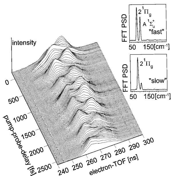
FIG. 2. The measured time-of-flight (TOF) photoelectron distribution as a function of pump-probe delay is shown. This femtosecond time-resolved photoelectron signal shows the vibrational wave-packet motion on the neutral electronic states. Cuts at a constant TOF reveal the wave-packet dynamics at a specific internuclear distance. The insets display the Fourier transform of transient photoelectron signals obtained at two different cuts. At an earlier TOF, photoelectrons with higher kinetic energy are released (“fast” photoelectrons) and therefore the inner turning point is probed, whereas at a later TOF the outer turning point is probed and “slow” photoelectrons are released. Consequently the Fourier transform of the “fast” photoelectron transient reflects wave-packet motion in the A^1\Sigma_u^+ and 2^1\Pi_g state, whereas the Fourier transform of the “slow” photoelectron transient reflects mainly the wave-packet motion in the 2^1\Pi_g state.
