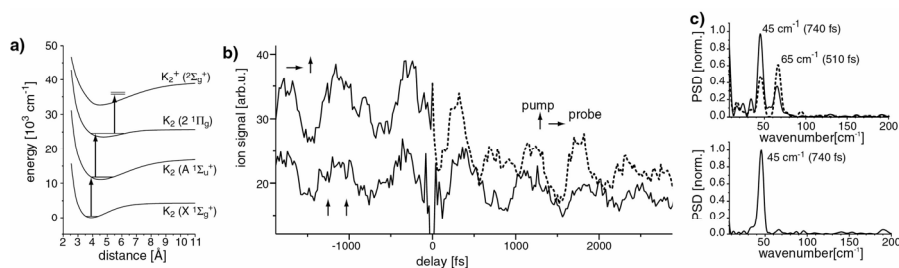
Fig. 1. a) Calculated potential energy curves of the potassium dimer system. b) Section of pump–probe transients with mutually parallel (solid line) and crossed (dashed line) linear polarizations around delay time zero. c) FFT-analysis of pump–probe transients with parallel (lower graph) and crossed (upper graph) mutual polarizations.
