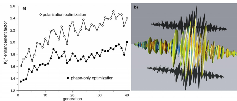
Fig. 2. a) Evolution curves show the K_2^+ ion yield relative to that obtained with an unshaped laser pulse. b) Quasi-three-dimensional representation of the optimal polarization-shaped laser pulse. Time evolves from -1.5\text{ps} (left) to +1.5\text{ps} (right), and electric field amplitudes are indicated by the sizes of the corresponding ellipses. The momentary frequencies are indicated by colors and the shadows represent the amplitude envelopes of the two orthogonal components.
