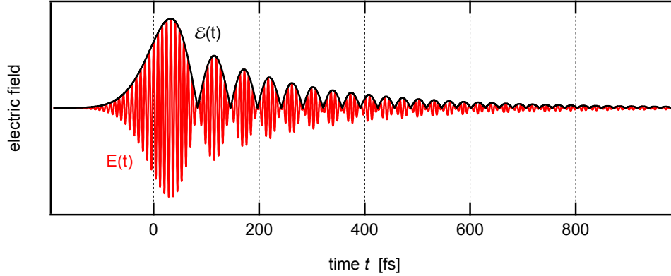
FIGURE 3. Example of a \Delta t = 30 fs FWHM pulse subjected to Third Order Dispersion (TOD) of \phi_3 = 90000 \text{ fs}^3 . The pulse starts with an intense sub-pulse followed by a long pulse train. The statistical pulse duration \Delta t = \sqrt{8 \ln(2)} \sigma_t is 233 fs like in the GDD example in Fig. 1. For visualization purposes, the carrier frequency was chosen three times smaller than the actual carrier frequency (see above).
