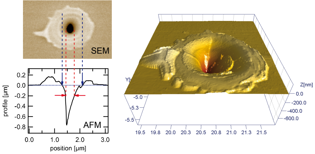
FIGURE 5. Left: SEM micrographs of a structure generated by positive TOD radiation with pulse energy twice above the threshold at \phi_3 = +6 \times 10^5 \text{ fs}^3 . The corresponding depth profile measured by AFM is shown below. In this publication the term inner diameter relate to the diameter where the height profile falls below the unperturbed surface level (blue arrows). Note that the clearly visible contrast change in the SEM micrograph results from the high aspect ratio of the hole (red arrows). This deep channel diameter stays remarkably stable with respect to energy variations. [14,15] Right: AFM micrograph corresponding to the SEM micrograph shown left.
