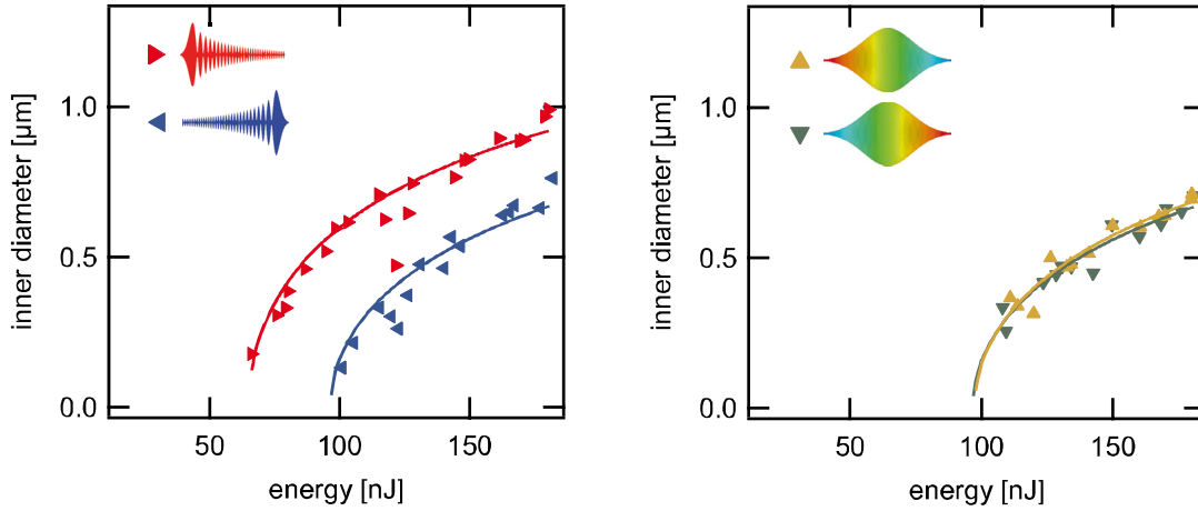
FIGURE 6. Left: (TOD) inner hole diameters of ablated structures for fused silica with \phi_3 = +6 \times 10^5 \text{ fs}^3 (red triangles) and \phi_3 = -6 \times 10^5 \text{ fs}^3 (blue triangles) measured by AFM. Right: (GDD) inner hole diameters of ablated structures for fused silica with \phi_2 = +1 \times 10^4 \text{ fs}^2 (orange triangles) and \phi_2 = -1 \times 10^4 \text{ fs}^2 (green triangles) measured by AFM.
