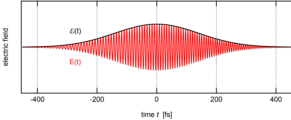
FIGURE 1. Example of a \Delta t = 30 \text{ fs} FWHM pulse subjected to a Group Delay Dispersion of \phi_2 = 2500 \text{ fs}^2 leading to an up-chirped pulse. In order to visualize the increase of the instantaneous frequency \omega(t) with time the carrier frequency was chosen three times smaller than the actual carrier frequency of \omega_0 \approx 2.35 \text{ fs}^{-1} corresponding to a wavelength of 800 nm. The FWHM of the spectral energy bandwidth is \Delta\varepsilon = 60.8 \text{ meV} . The pulse is Gaussian in shape with a pulse duration of 233 fs (FWHM of the intensity).
