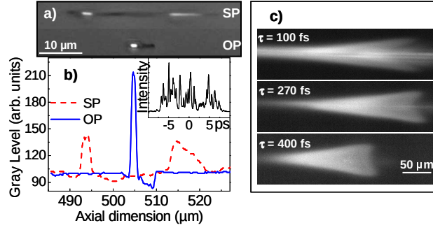
Fig. 5.13. (a) Short pulse (SP) and optimal pulse (OP) induced structures at a depth of 500 \mu\text{m} and 1 \mu\text{J} input energy indicating the spatial confinement of the OP structure in the presence of aberrations. (b) The corresponding axial cross-sections. The inset shows the optimal pulse shape [86]. (c) Control of spatial distribution of excitation using the pulse duration [87]. Plasma emission images recorded in waveguide writing conditions in phosphate glass using different laser pulse durations and a slit shaping technique. Beam filamentation and prefocal energy depletion are minimized for circular polarization and increasing pulse durations
