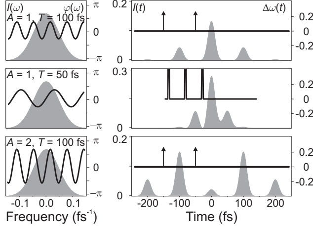
Fig. 5.3. Upper panel: sinusoidal spectral phase modulation with A = 1 ; T = 100 \text{ fs} , \phi = 0 . Middle: lowering the modulation frequency to T = 50 \text{ fs} merges the sub-pulses. Increasing the amplitude A results in a higher number of sub-pulses. The arrows indicate again a phase change by \pi
