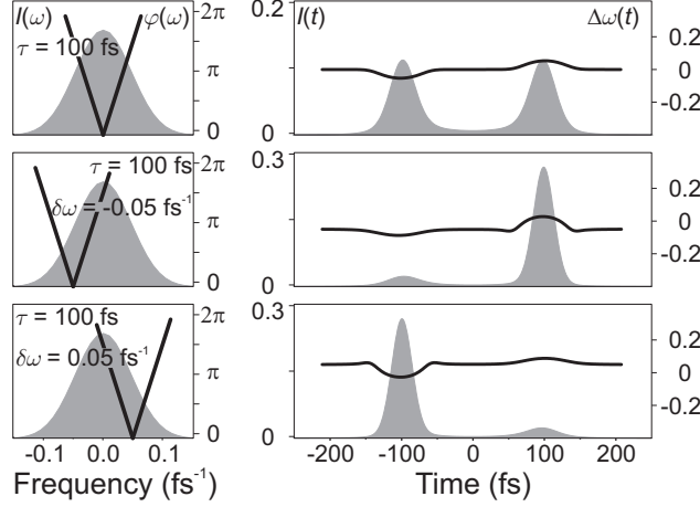
Fig. 5.5. An upright V-shaped spectral phase \varphi(\omega) = \tau |\omega - \delta\omega| creates a sequence of a red-detuned pre-pulse and a blue-detuned post-pulse: each portion of the spectrum where the phase is linear corresponds to a longer pulse shifted by \pm\tau
