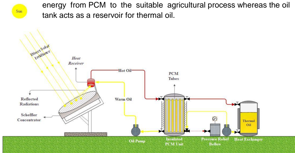
Experimental Setup of Latent Heat Thermal Energy Storage System
