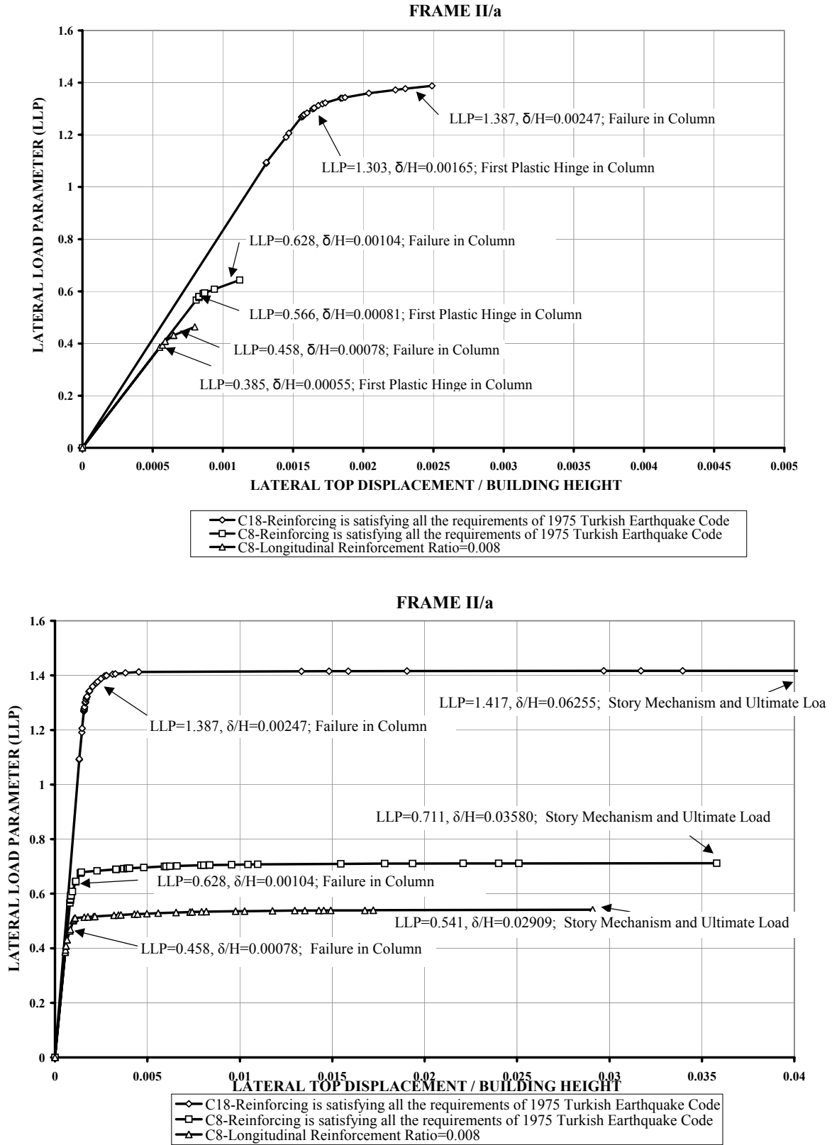
Figure 3.5.(f) Structural behaviors of the low rise reinforced concrete buildings
