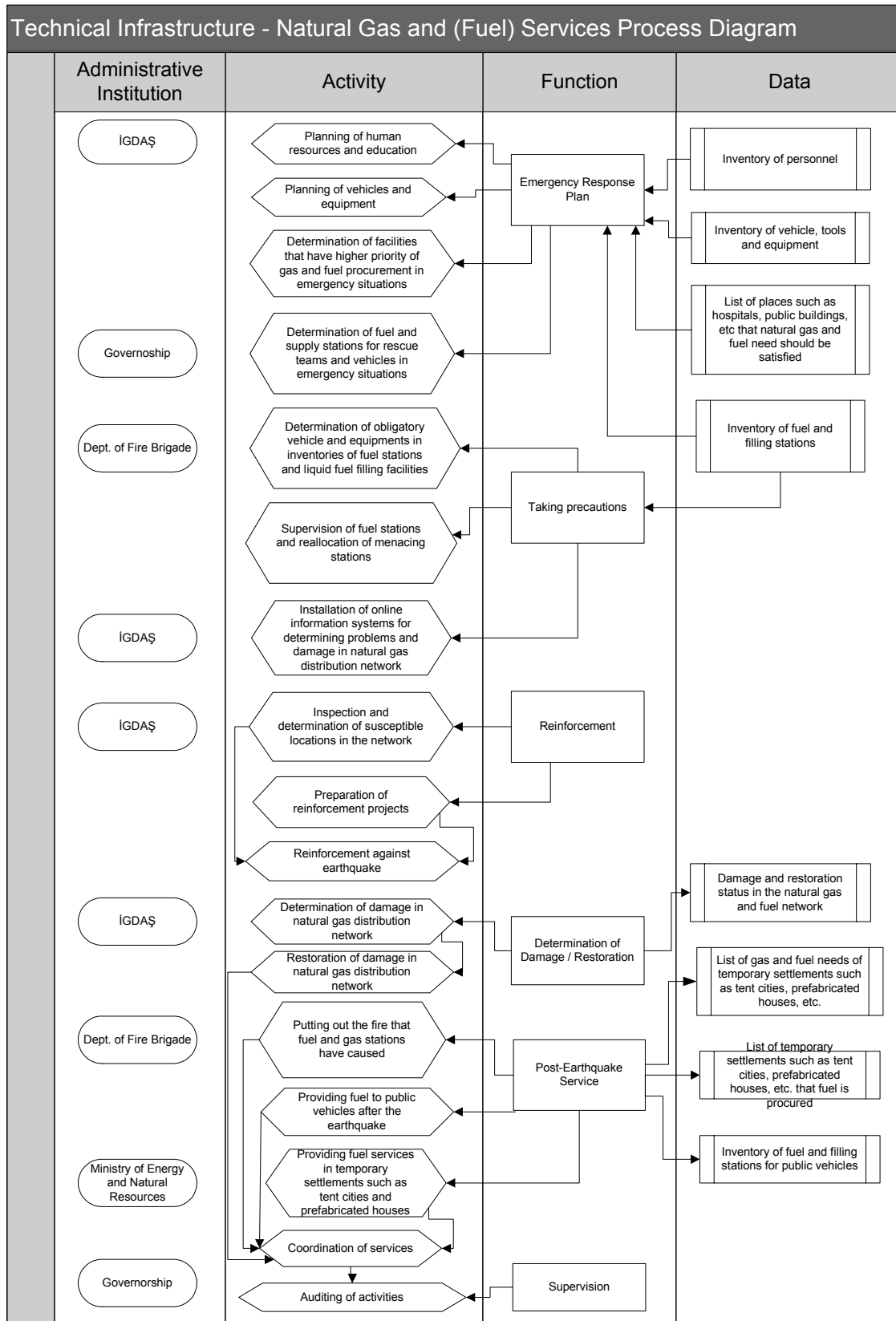
Figure 7.1.6. Process diagram of technical infrastructure – Natural gas and fuel services
