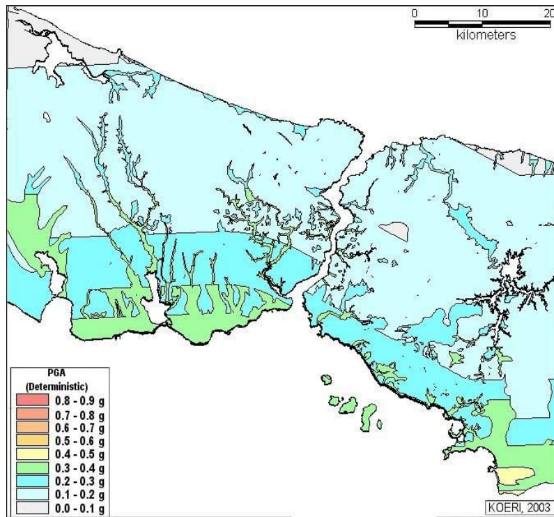
Figure 2.1.3. Site dependent deterministic peak ground accelerations
