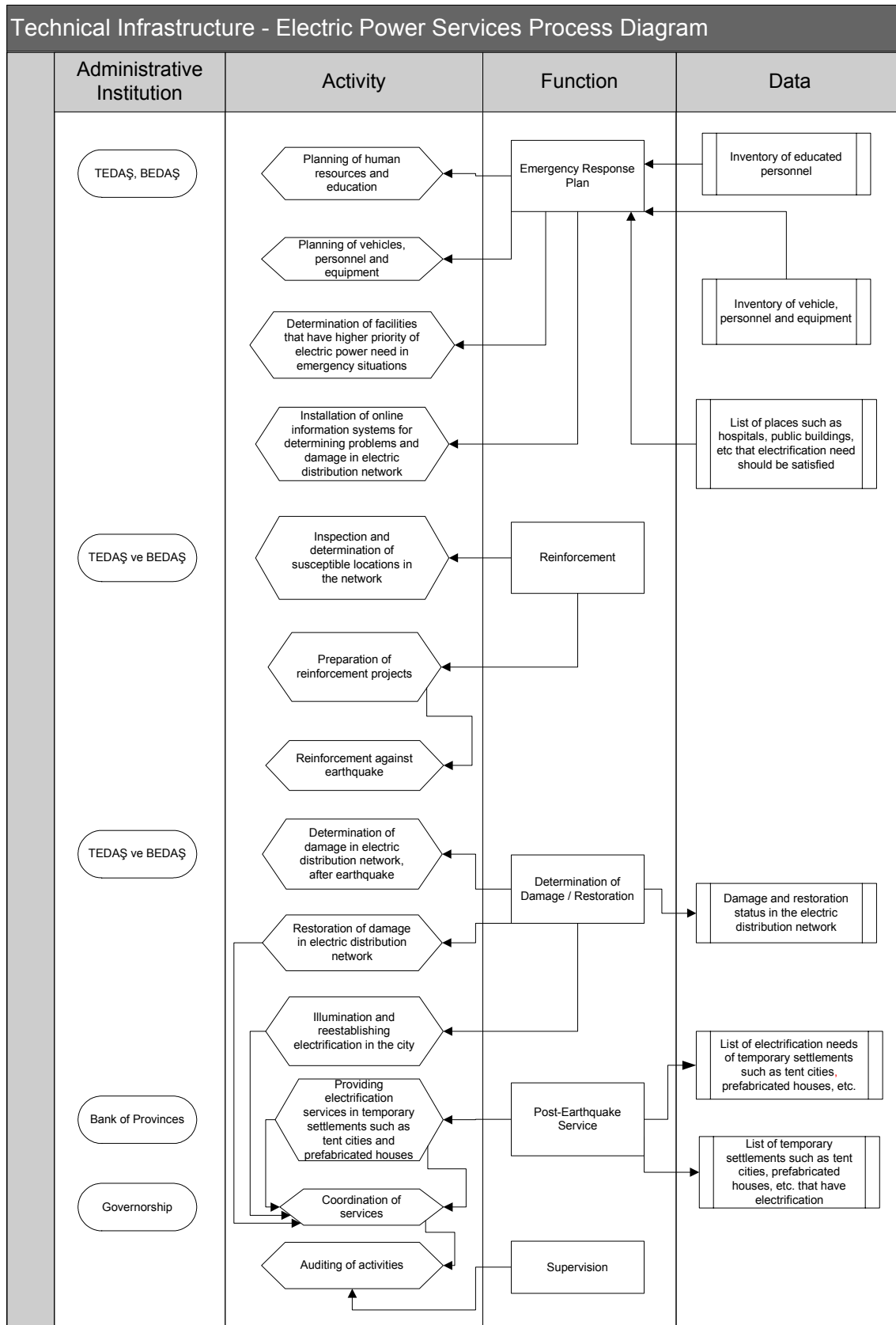
Figure 7.1.5. Process diagram of technical infrastructure – Electric and power services
