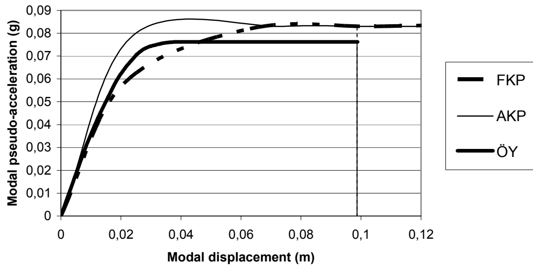
Figure E5b. Capacity diagrams in Y-Y direction (Coloumn mechanism: 4 storey building)
