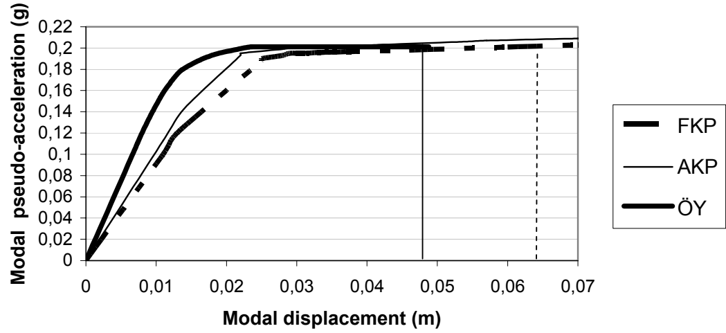
Figure E4b. Capacity diagrams in X-X direction (Beam mechanism: 4 story building)
