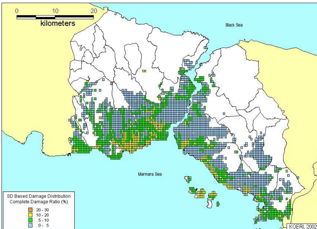
Figure 2.1.18. Ratio of the collapsed buildings to the total number of buildings (based on the scenario earthquake and spectral displacement based vulnerability curves, BU – ARC study)
