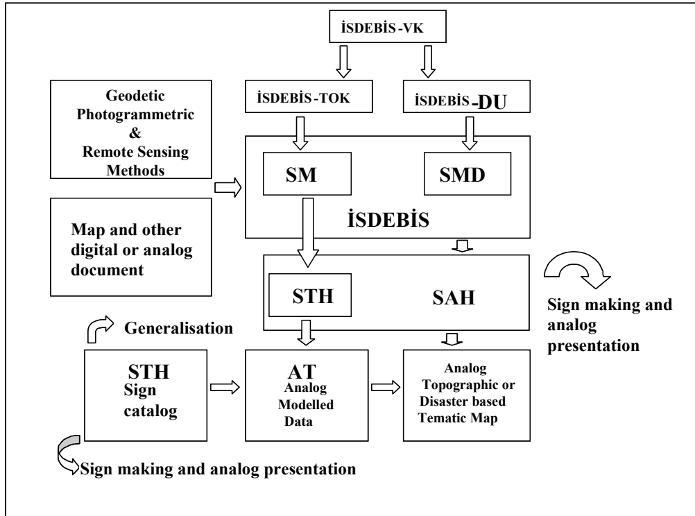
Figure 5.2.2: Modeling approach of spatial of ISDEBİS-TOK
