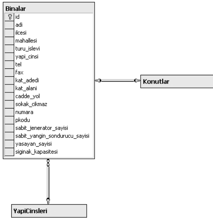
Figure 5.1.14. Building database in table form
