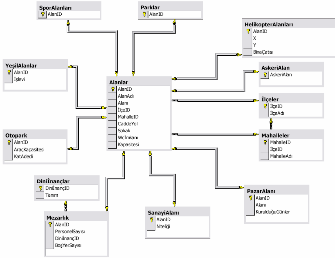
Figure 5.1.8. Proposed area database
