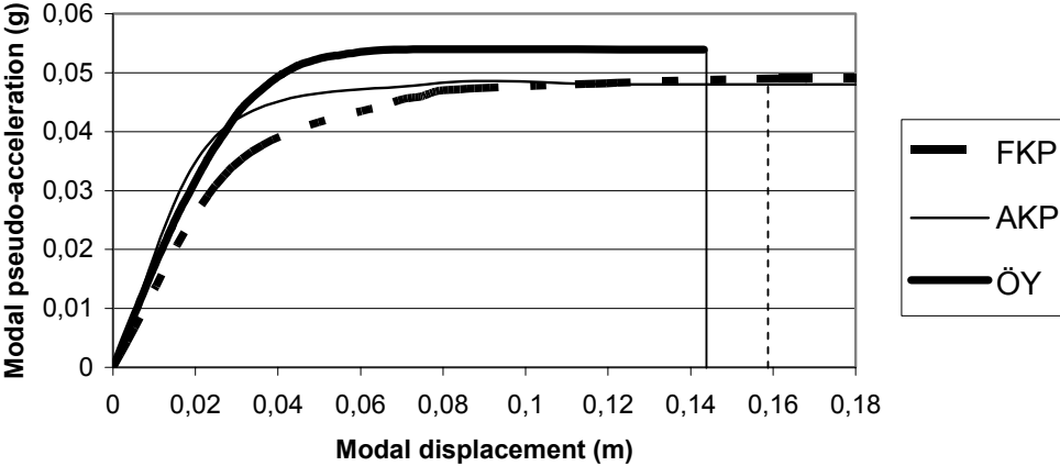
Figure E5d. Capacity diagrams in Y-Y direction (Column mechanism:6 storey building)
