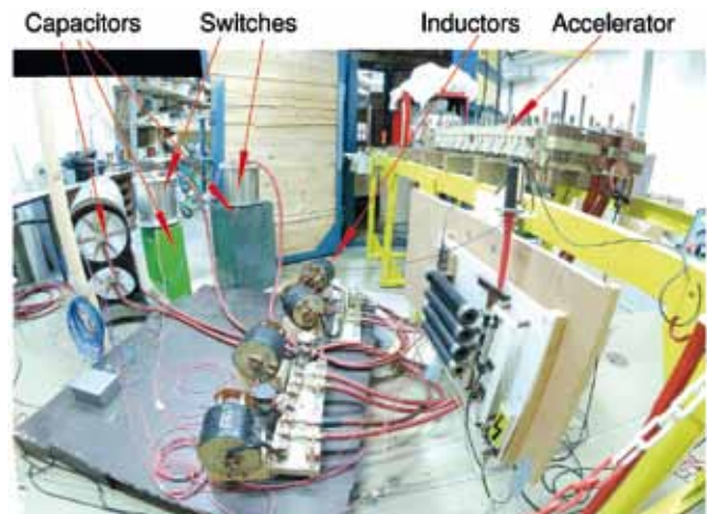
Experiment: Taylortest Rail Gun Experimental Setup: Taylor Test Rail Gun
