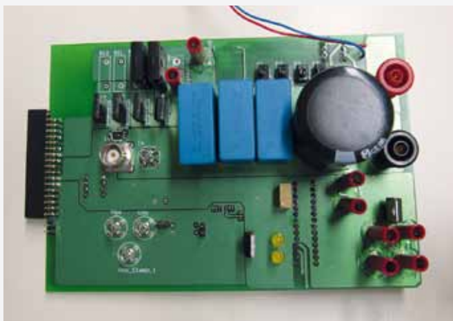
Platine des dynamischen Testsystems Board of the dynamic test system
