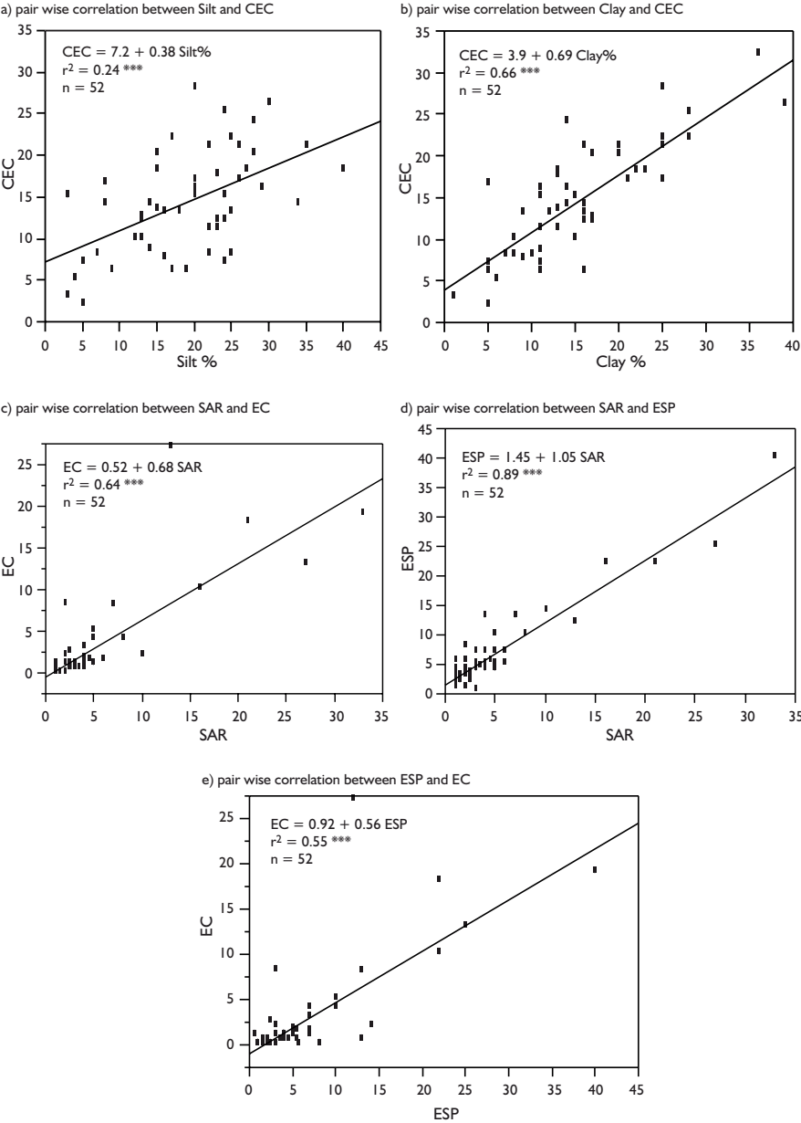
Figure 1: Pairwise correlations between different soil characteristics (depth 0-30 cm)
