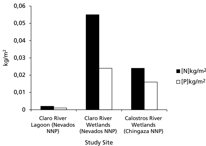
Figure 5: Relation between the concentration of N and P ( \text{kg/m}^2 ) and the study sites ( p=0.013 , CI = 95%).
