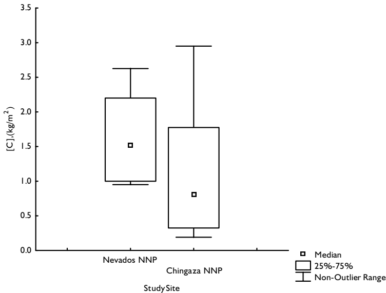
Figure 4: Relation between concentrations of carbon (kg/m 2 ) at the study sites (Nevados and Chingaza).
